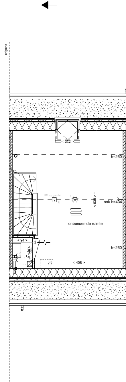
zolder
